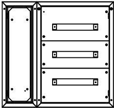
VISTA FRONTAL INTERNA NWP-3-DG-S+NWP-318-S
