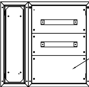
VISTA FRONTAL INTERNA NWP-3-DG-S+NWP-318-S COM TAMPA CEGA
