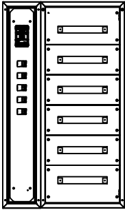
VISTA FRONTAL INTERNA NWP-6-DG-S + NWP-618-S COM TAMPAS ABERTAS
