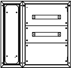
VISTA FRONTAL EXTERNA COM TAMPA CEGA NWP-3-DG-S+NWP-318-S
